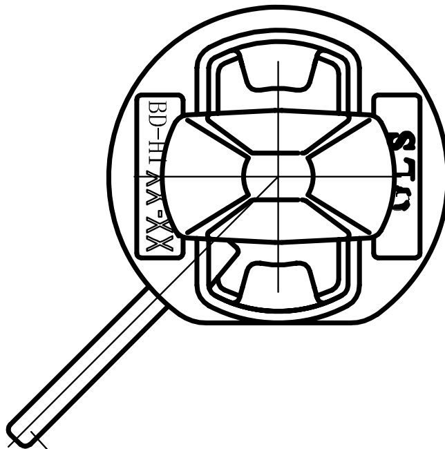
左旋锁锁紧时手柄位置 POSITION OF HANDLE WHILE LOCKING, LEFT TWISTLOCK
