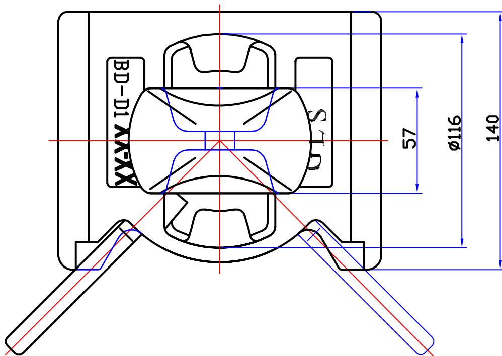
POSITION OF LEFT TWISTLOCK HANDLE WHILE LOCKING
